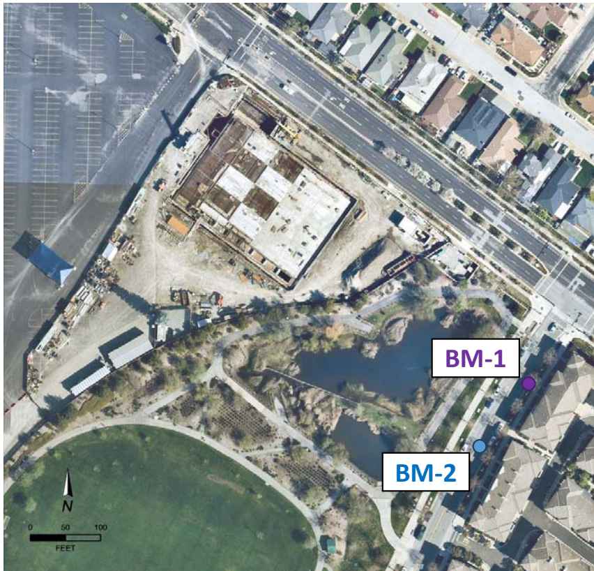
Approximate Locations of Bay Meadows Piezometers BM-1 and BM-2
